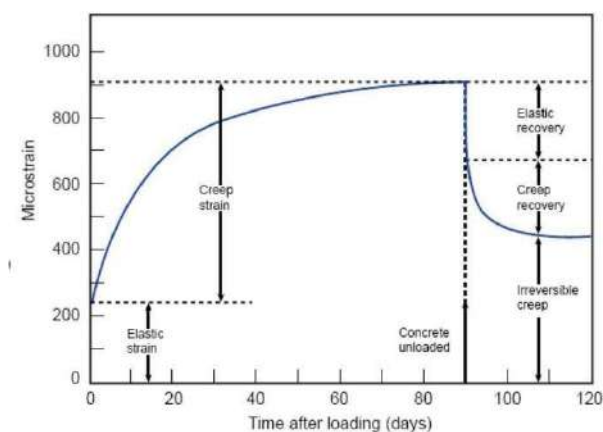
Fig 39: Microstrain curve
