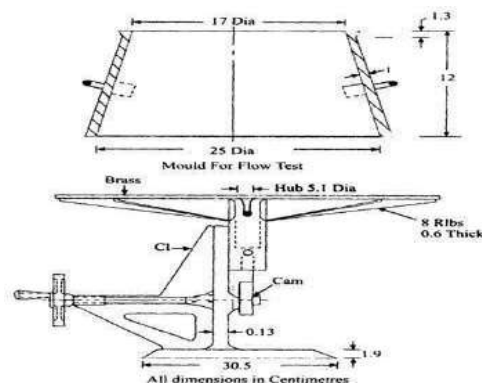
Fig 21: Flow table test
